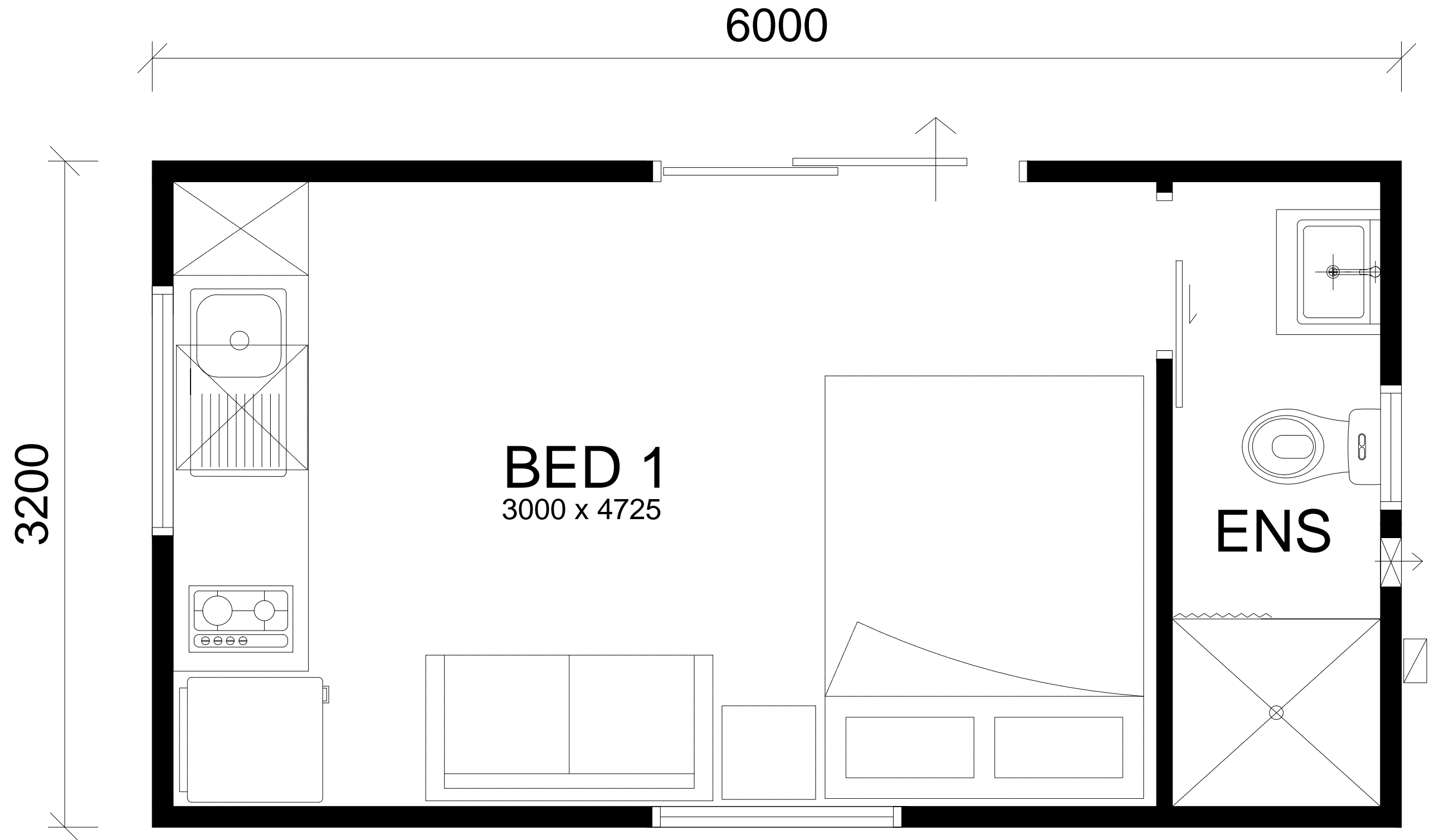
FLOOR PLAN - 6 x 3.2
