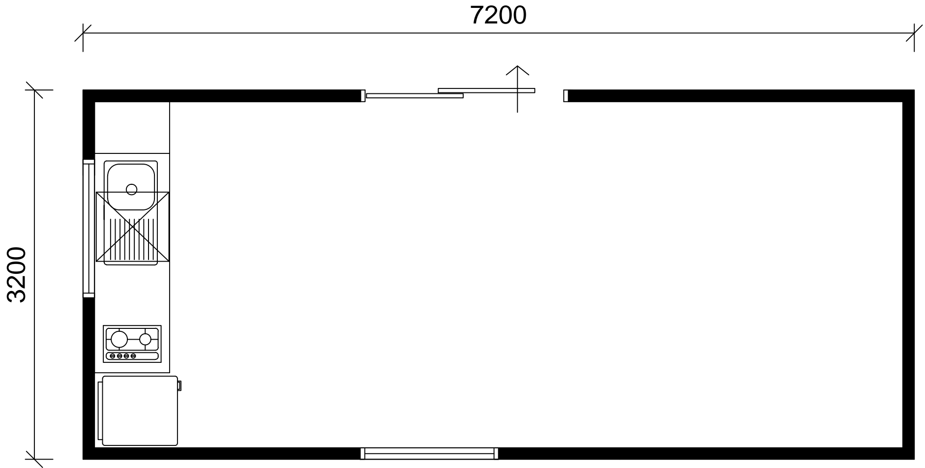
FLOOR PLAN - 7 x 3.2
