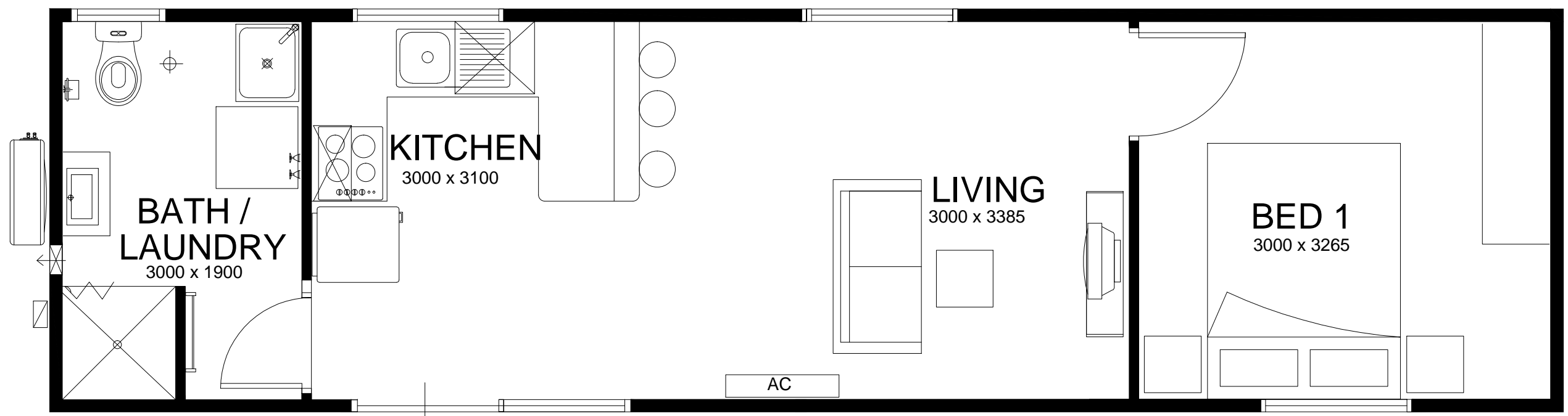
FLOOR PLAN - 12 x 3.2
